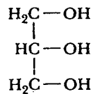
Glycerol
